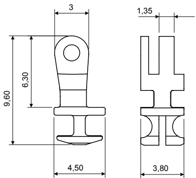
90° INSERT HINGE 03MACF864A1BN0 Material: Nickel silver
