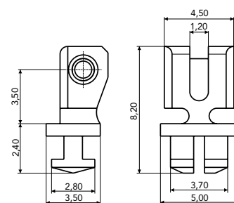
90° INSERT HINGE 03FRA0262A1BN0
