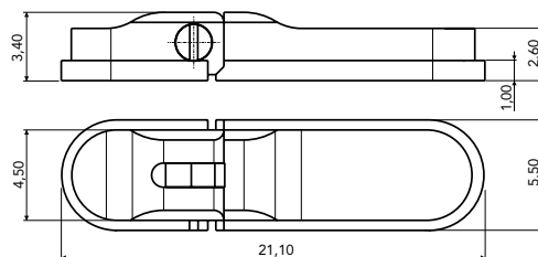
ASSEMBLED HINGE 03ELA0173A1BN0
