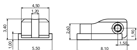
180° FRONT HINGE 03FRA0171A1BN0
