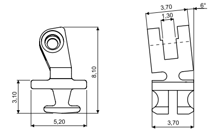
90° INSERT HINGE 03FRC4140A2BN0 Material: Nickel silver ADJUSTABLE 6° SLANTED ANGLE
