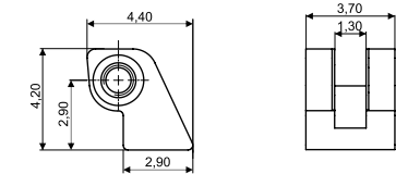
STEP HINGE 03FRC4162A1BY0 Material: Nickel silver
