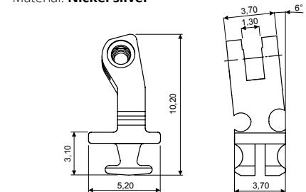
90° INSERT HINGE 03FRC4156A2BN0 Material: Nickel silver HIGH VERSION ADJUSTABLE 6° SLANTED ANGLE
