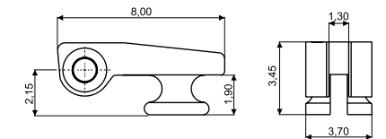
180° INSERT HINGE 03FRC4145A2BN0 Material: Nickel silver
