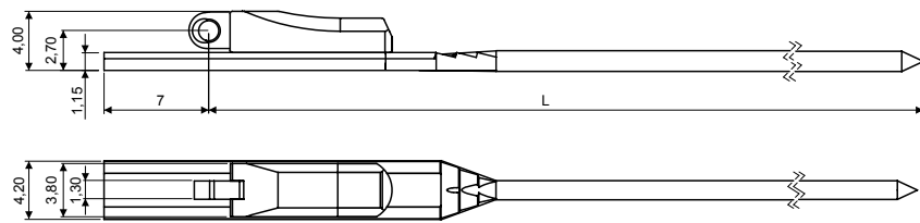
WIRECORE L 130 03WFC6107A130BNX L 135 03WFC6107A235BNX Material: Nickel silver Trolley: Hard Trolley Note: Soft Trolley available on request
